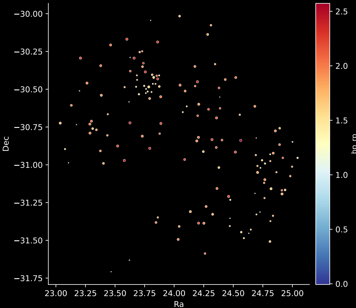
APOGEE DR17 Field: [Sgr_rvvar2] Stars: 145
