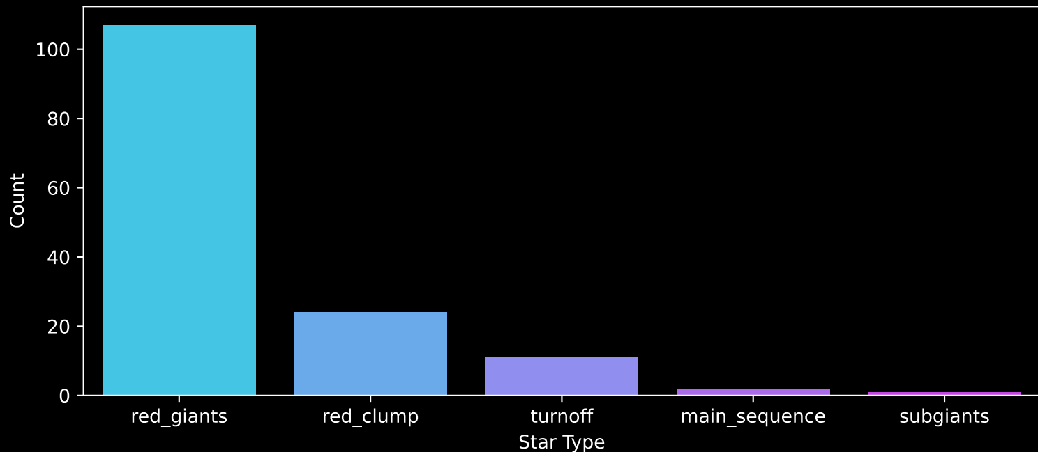
APOGEE DR17 Field: [Sgr_rvvar2] Count plot of Star Type
