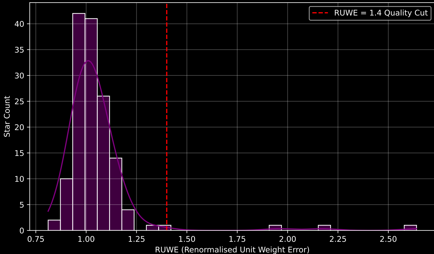
GAPOGEE DR17 Field [Sgr_rvvar2] RUWE Distribution (n= 144)
