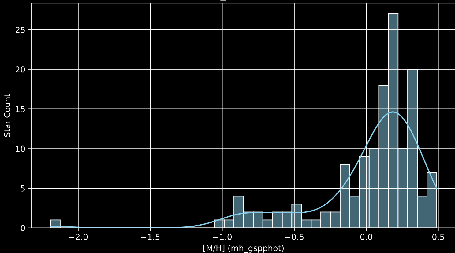
APOGEE DR17 Field: [Sgr_rvvar2 [M/H] (mh_gspphot) (n= 142)
