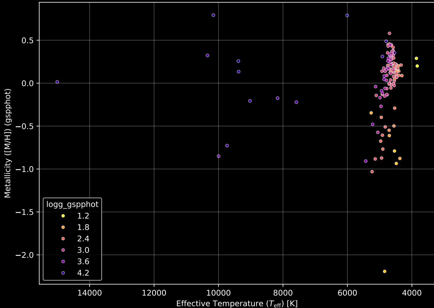
APOGEE DR17 Field: [Sgr_rvvar2] Stellar Population Parameters (n= 145)
