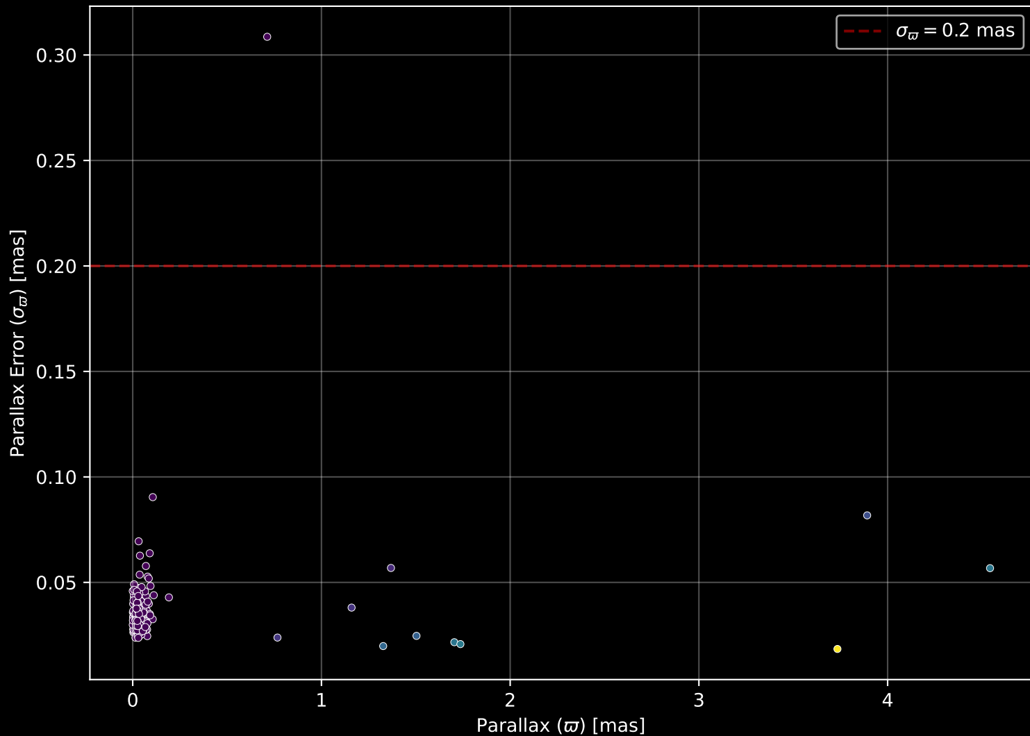
APOGEE DR17 Field: [Sgr_rvvar2] Parallax Quality (n= 145)
