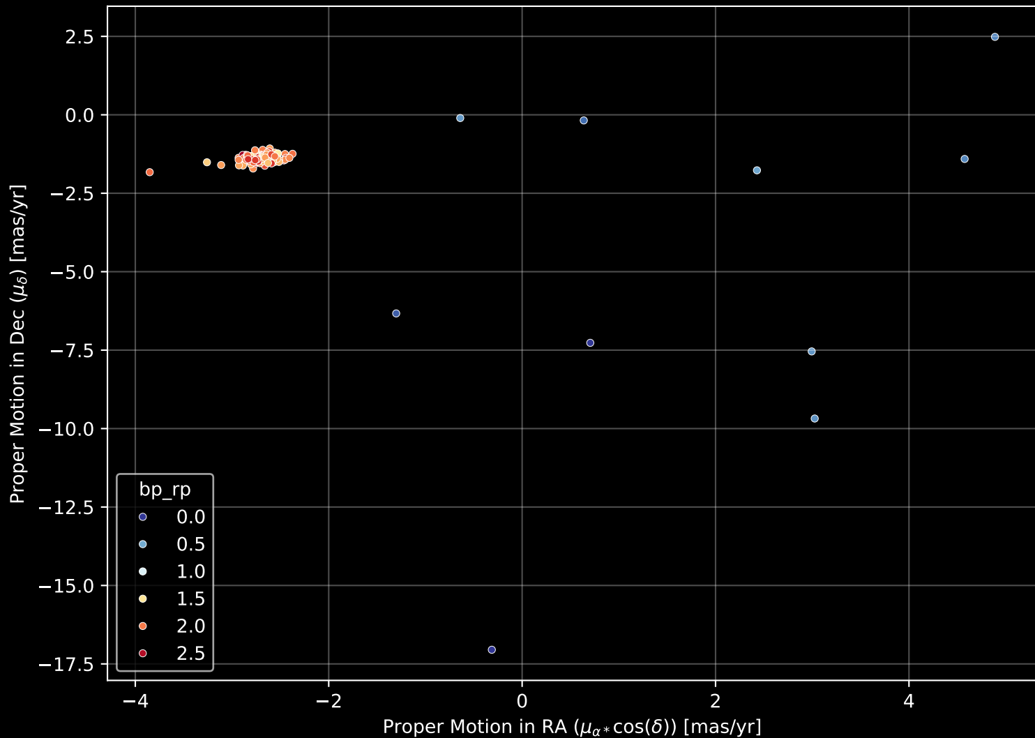
APOGEE DR17 Field: [Sgr_rvvar2] Proper Motion Diagram (n= 145)
